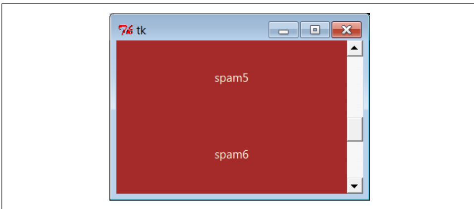
Figure 9-24. scrolledcanvas live
